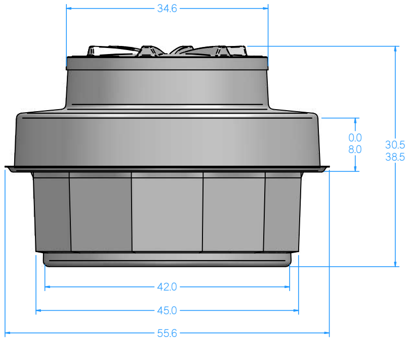
PC4540U ASSY
