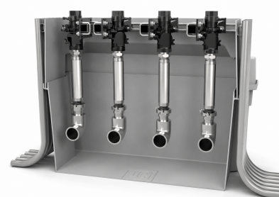
Height-adjustable riser.
